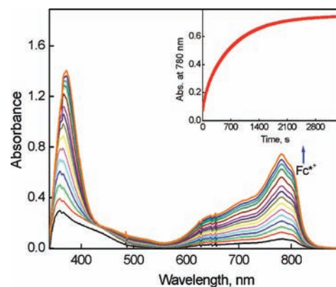
Figure 1. UV–vis spectral changes observed in the two-electron reduction of \text{O}_2 catalyzed by [\text{Cu}^{\text{II}}_2(\text{LO})(\text{OH})] (D1) ( 0.040 \text{ mM} ) with \text{Fc}^* ( 1.0 \text{ mM} ) in the presence of HOTF ( 3.0 \text{ mM} ) in \text{O}_2 -saturated acetone ( [\text{O}_2] = 11.0 \text{ mM} ) at 223 K. The inset shows the time profile of the absorbance at 780 nm due to \text{Fc}^{*+} .
