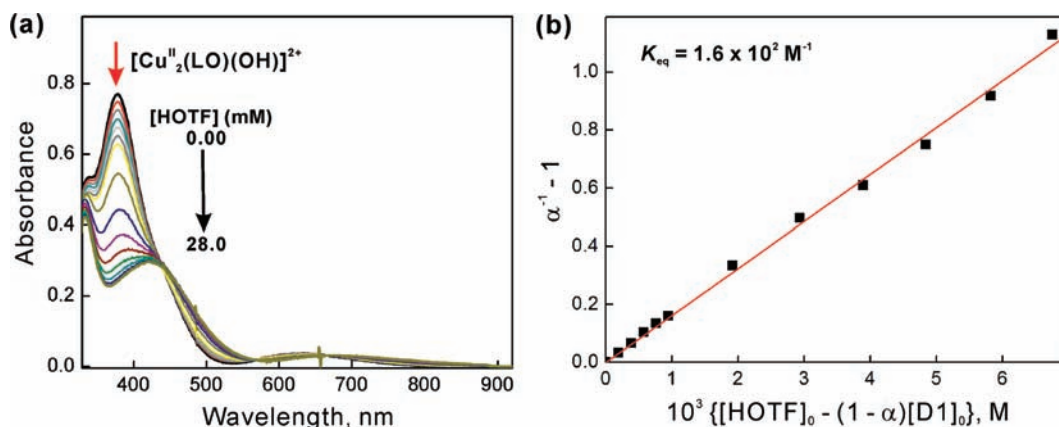
Figure 3. (a) UV–visible spectral changes of [\text{Cu}^{\text{II}}_2(\text{LO})(\text{OH})] ( D1 ) (0.20 mM) in the presence of HOTF (0.0–28.0 mM) in acetone at 298 K. (b) Plot of \alpha^{-1} - 1 versus \{[\text{HOTF}]_0 - (1 - \alpha)[\text{D1}]_0\} to determine the equilibrium constants ( K_{\text{eq}} ) in the protonation of D1 upon addition of TFA (0.0–28.0 mM) into the solution of D1 (0.20 mM) in acetone at 298 K.
