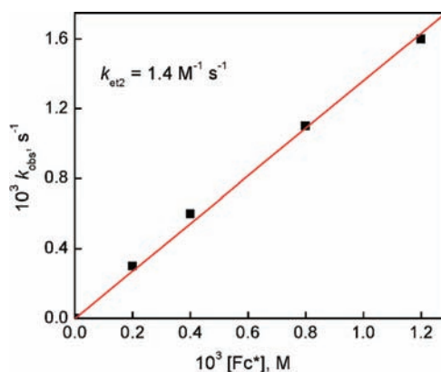
Figure 9. Plot of the pseudo-first-order rate constants ( k_{\text{obs}} ) versus concentrations of \text{Fc}^* in the second electron transfer from \text{Fc}^* to [\text{Cu}^{\text{II}}\text{Cu}^{\text{I}}(\text{LO})]^{2+} ( D2 ) (0.10 mM) to determine the k_{\text{et2}} value in the presence of HOTF (2.0 mM) in acetone at 213 K.
